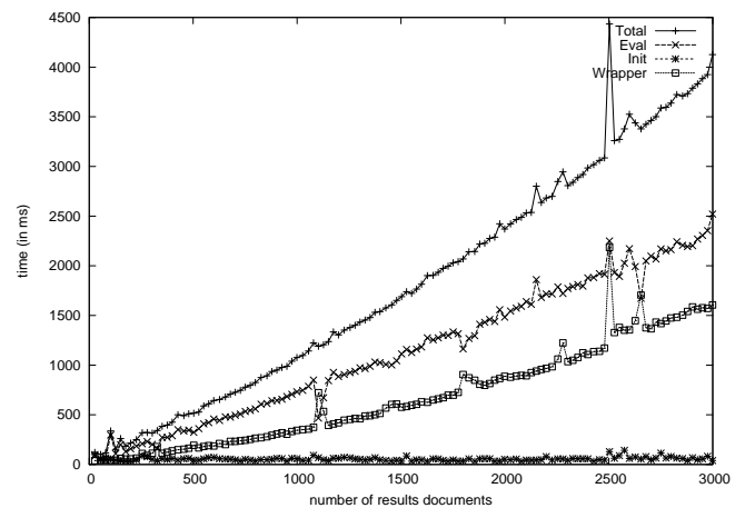
Figure 3: Execution time for each step
